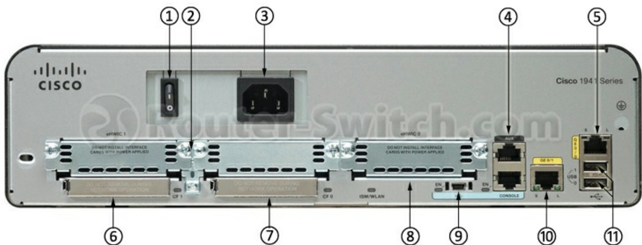
Figure 4 shows the ports and slots on the back panel of Cisco 1941/K9.
