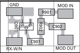
ADDITIONAL PCB
