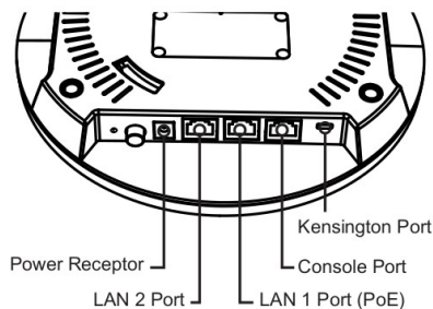
Figure 2. DWL-7620AP Rear Panel
