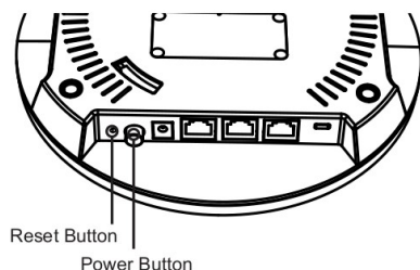
Figure 2. DWL-7620AP Rear Panel
