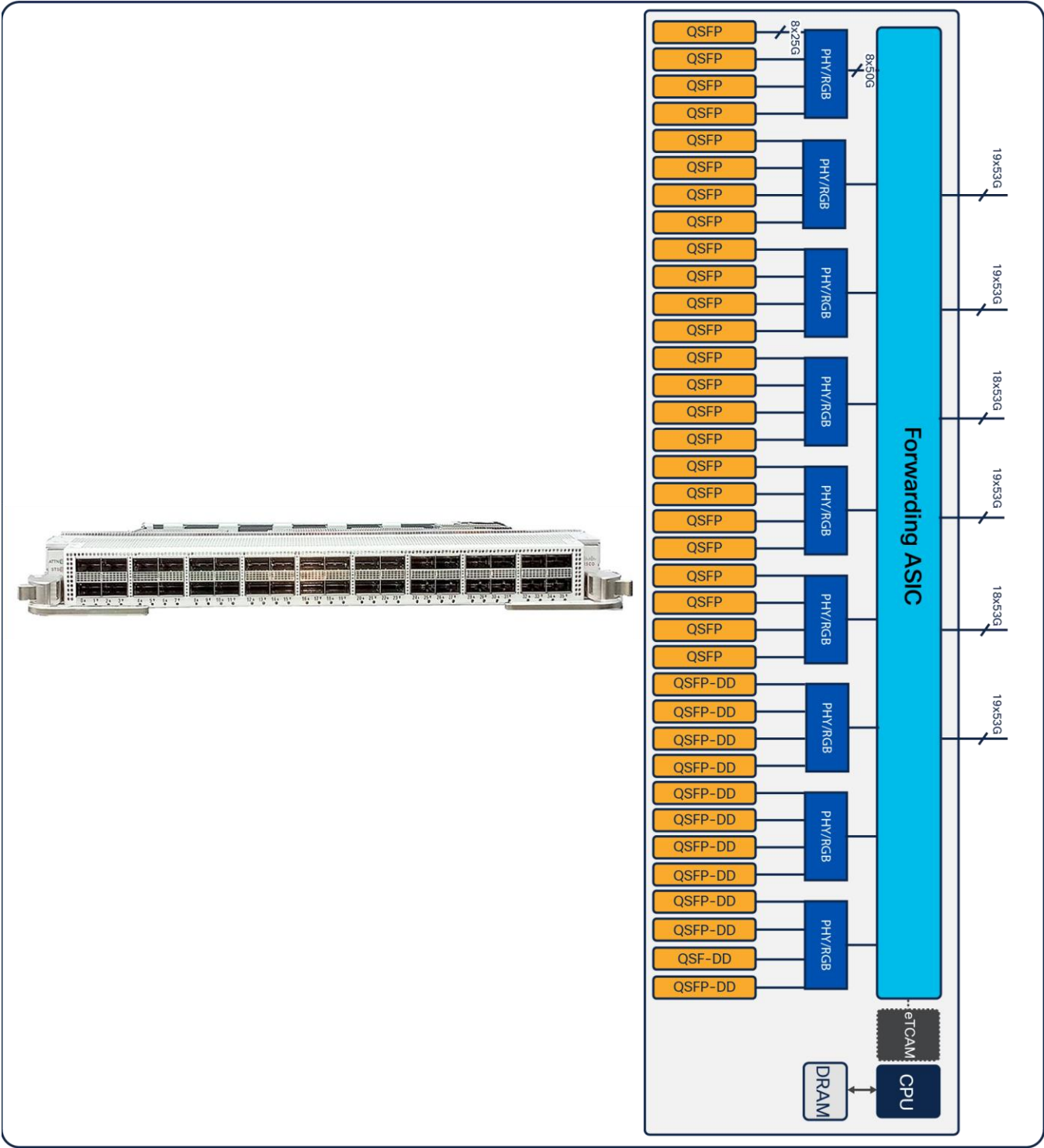
Figure 24. NCS 5700 36x 100G scale line card
