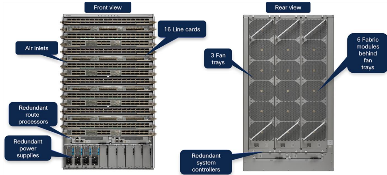
Figure 3. NCS 5516 chassis front view and rear view
