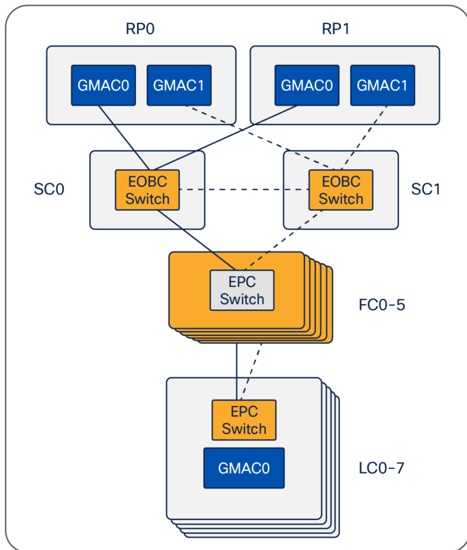
Figure 10. EPC network
