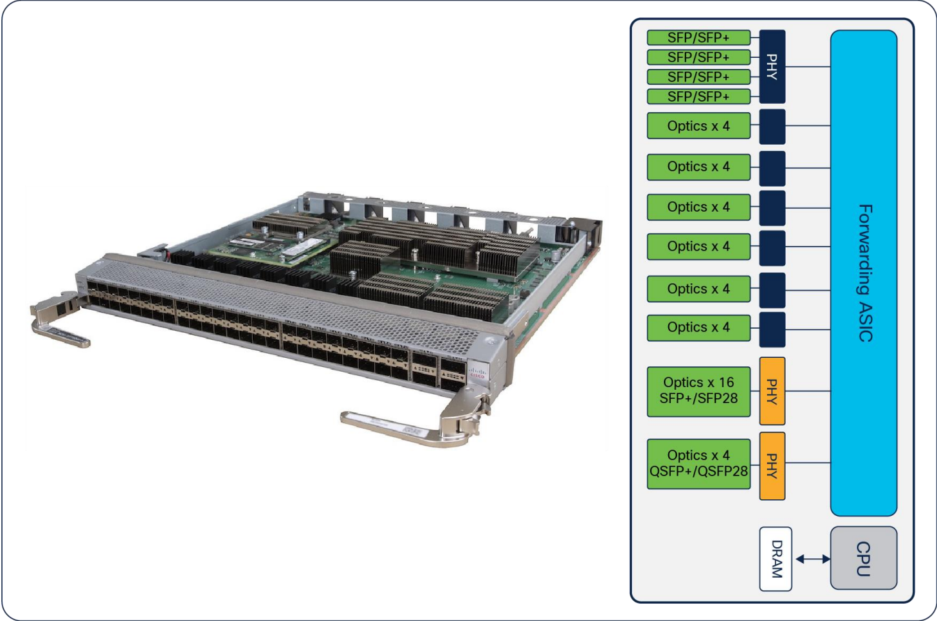
Figure 29. NCS 5500 32x10G 16x25G 4x100G base line card
