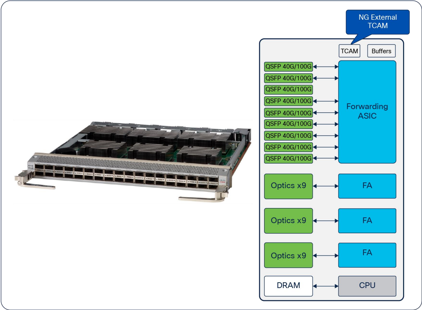
Figure 26. NCS 5500 36x 100G scale line card
