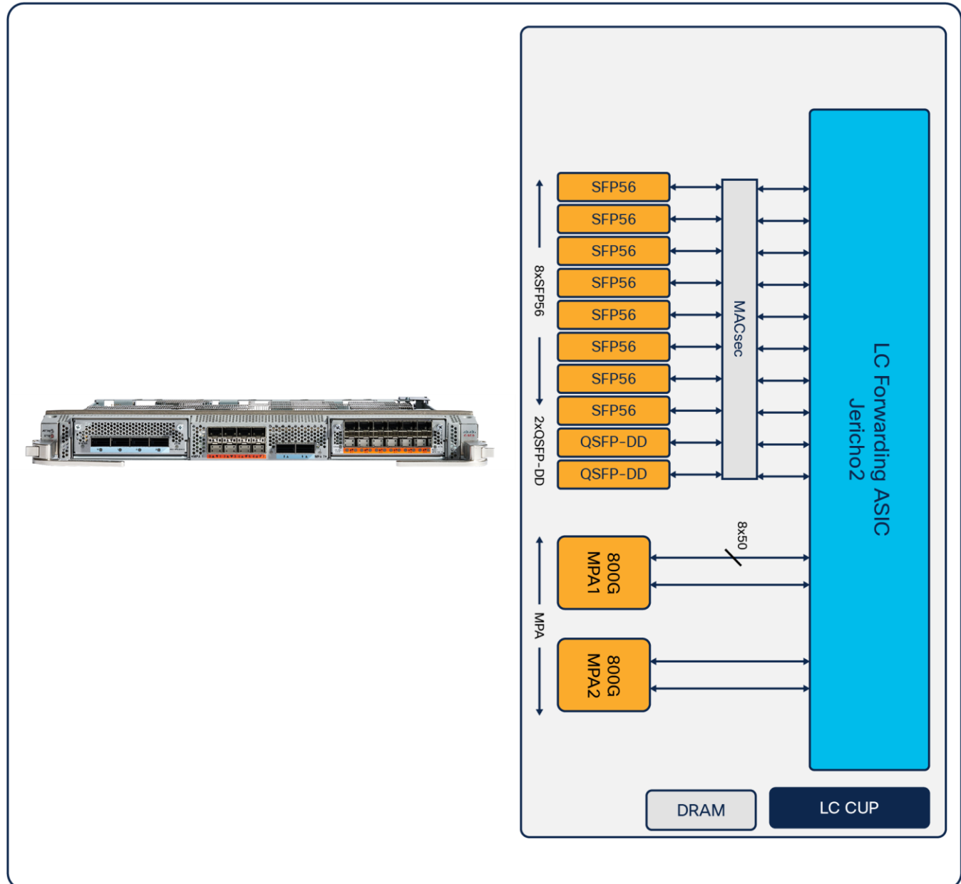
Figure 25. NC57-MOD-S base line card
