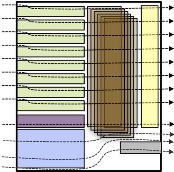
Figure 15. NCS 5508 front to back airflow example
