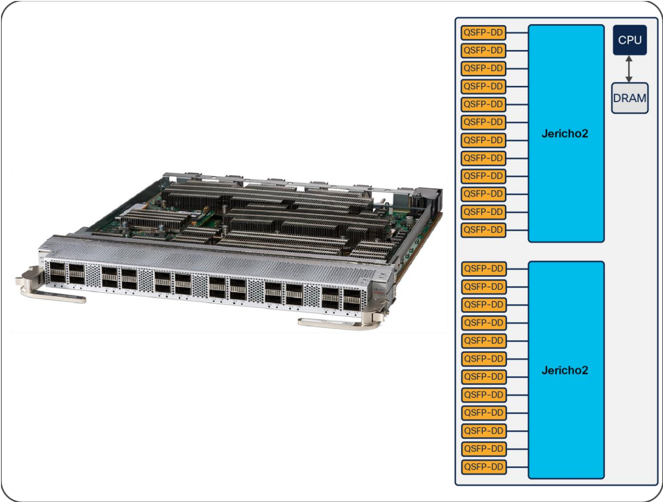
Figure 21. NCS 5700 24x400G base line card
