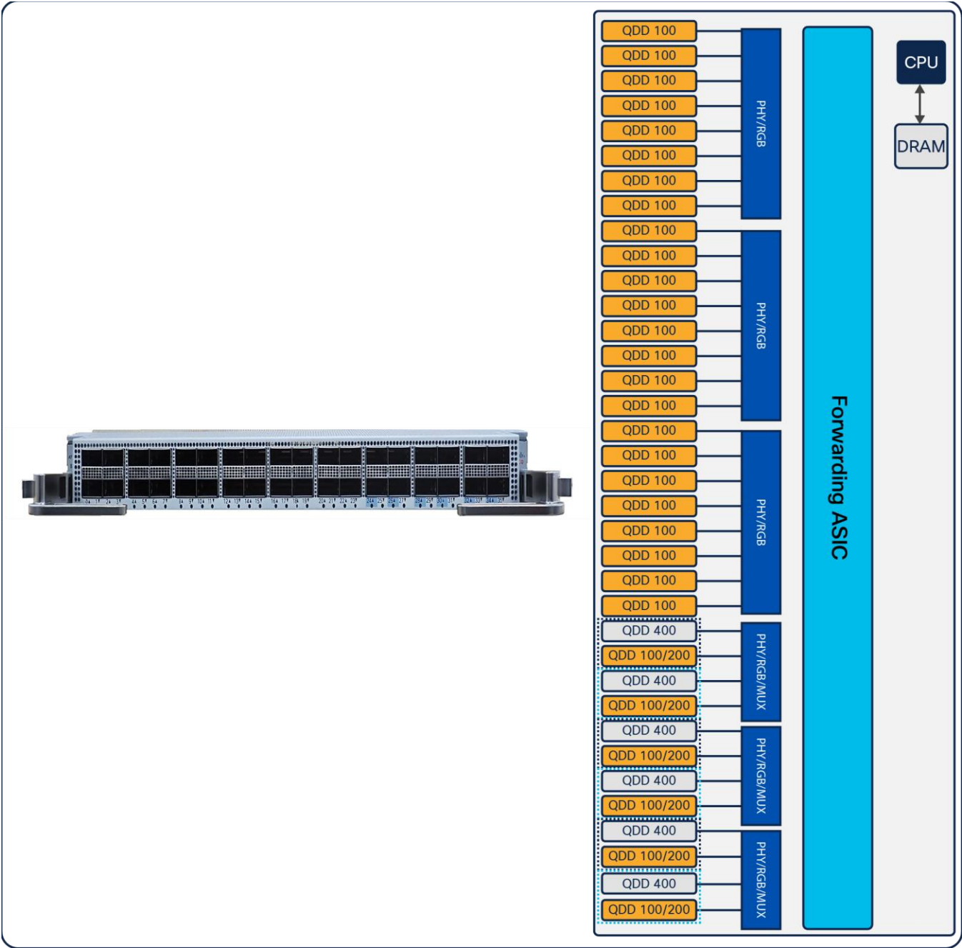
Figure 23. NCS 5700 36x 100G base line card
