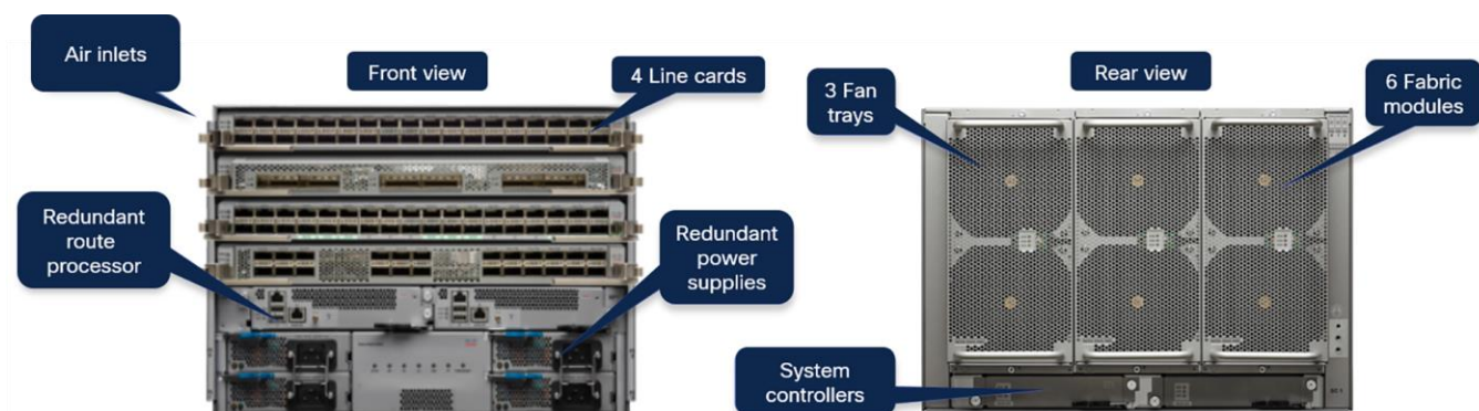
Figure 1. NCS 5504 chassis front view and rear view
