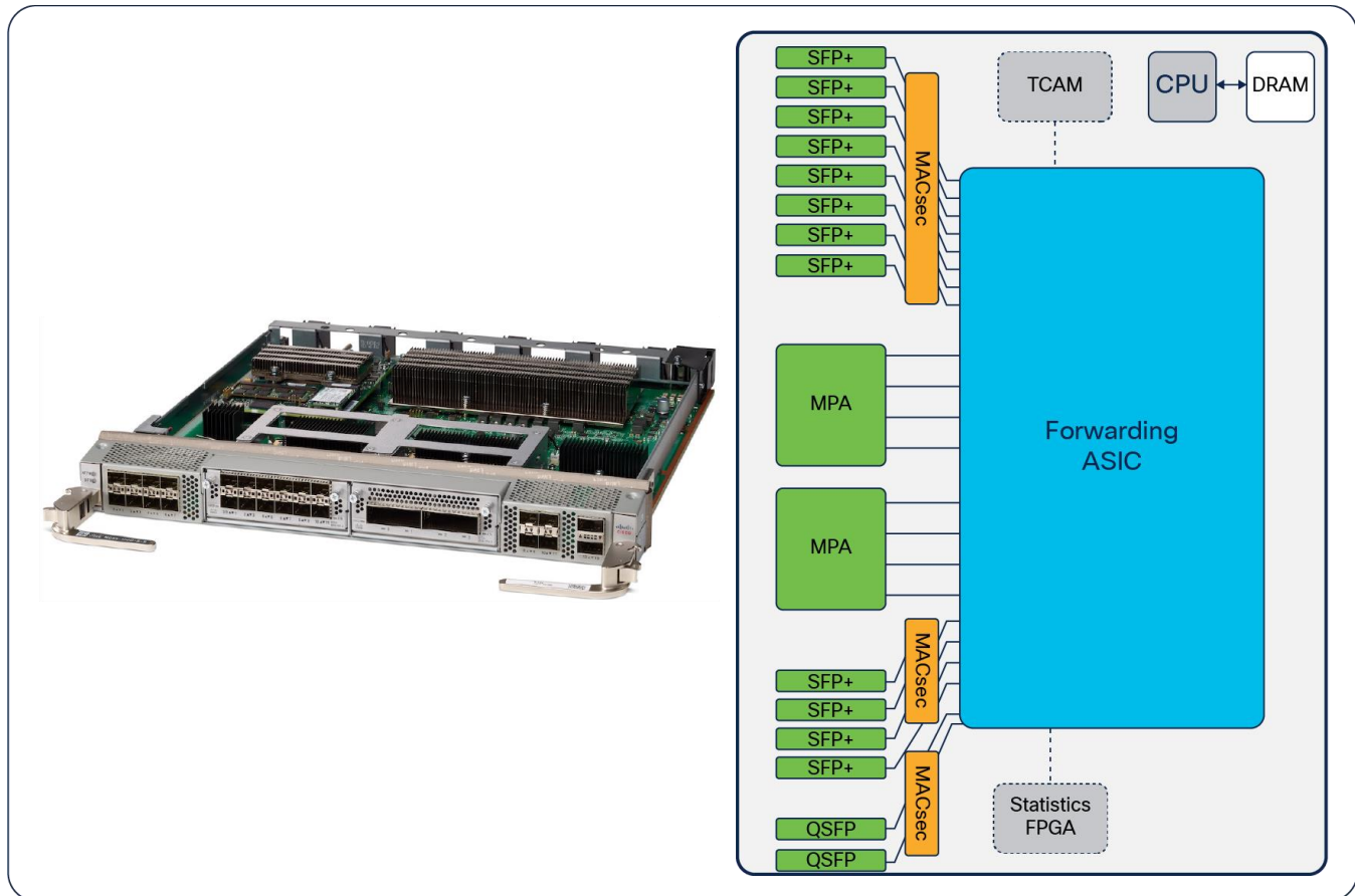
Figure 28. NCS 5500 MOD base and scale line card
